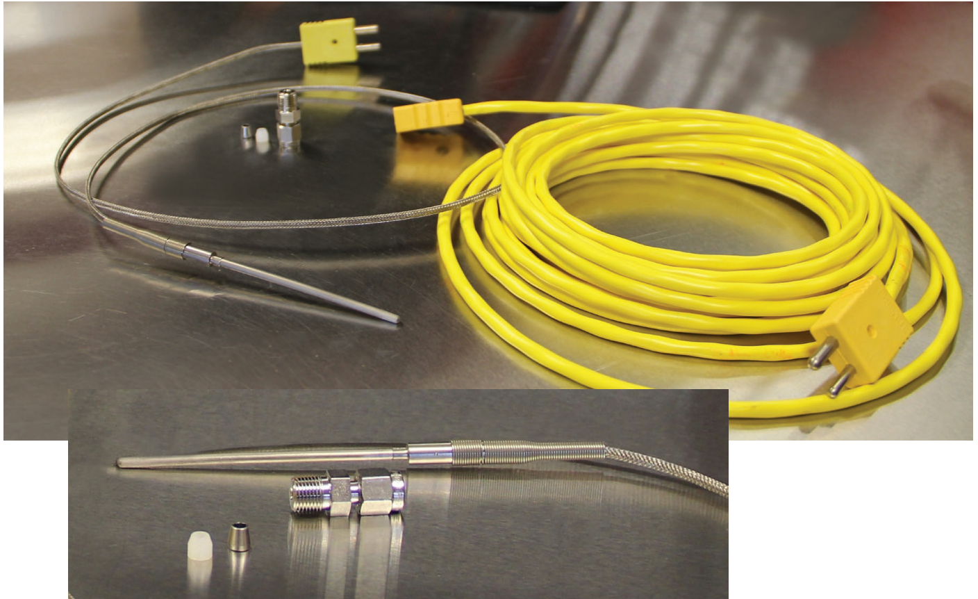
Type K Thermocouples, fittings and low and high temperature ferrules
